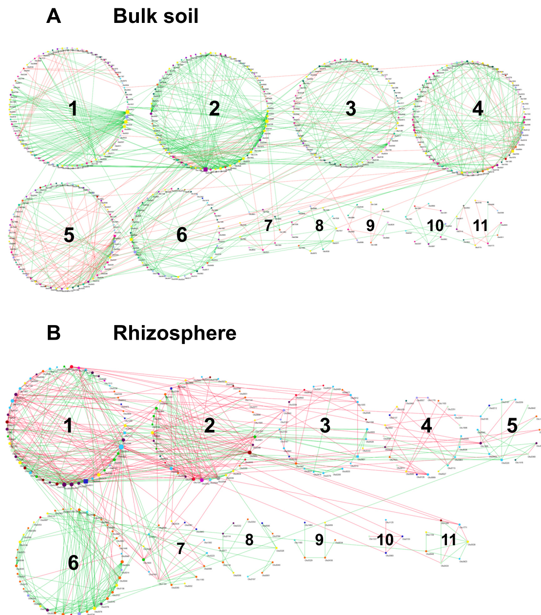
Fig. 3. Co-occurrence networks of total bacterial communities in bulk soil (A) and rhizosphere (B). Green and red lines connecting nodes indicate positive and negative interactions, respectively. Colour of nodes represent OTUs from different phyla. Square-shaped nodes represent module hubs. Numbers represent the modules.
