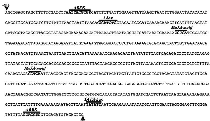
Figure 2. Nucleotide sequence of the promoter fragment corresponding to the Fahyprp gene. Upper bars indicate the putative cis -sequences found in the promoter fragment. ABRE is a putative abscisic acid cis element (Baker et al. , 1994; Hattori et al. , 1995), I-box is involved in the regulation by light (Yamaguchi-Hinozaki et al. , 1994), and putative MeJA-motif is linked to regulation by jasmonic acid pathway (Lee et al. , 1997).
