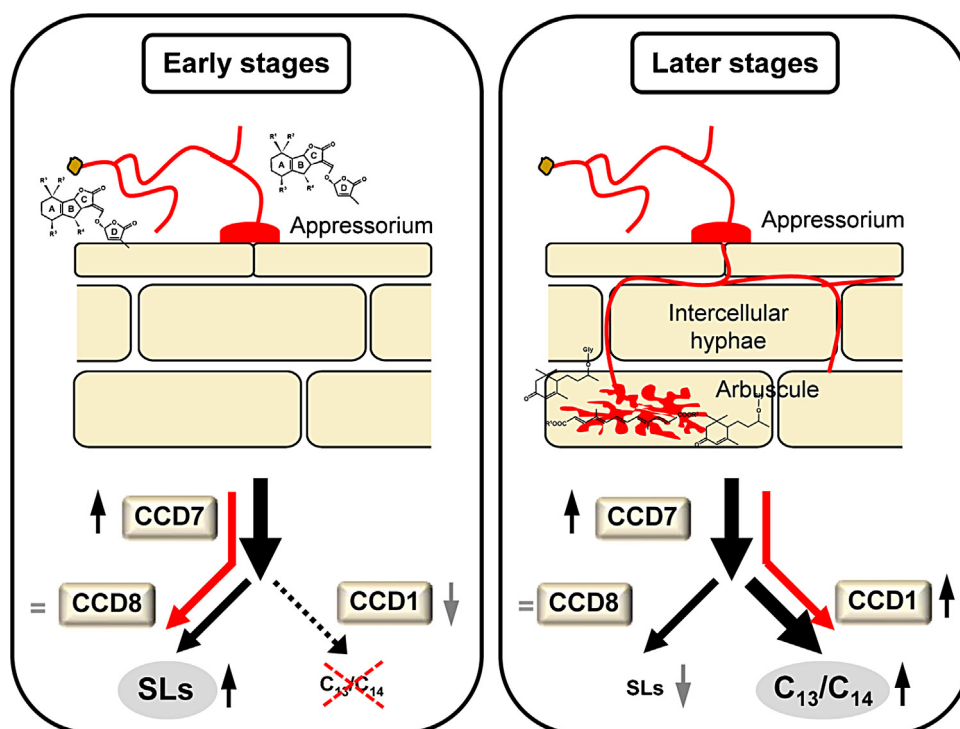
Fig. 7. Schematic summary of the host root colonization by AMF during the early and later stages. Induction of CCD7 promotes SL biosynthesis to favour host plant-AMF contact during the pre-symbiotic stage. During a well established symbiosis, induction of both CCD7 and CCD1 derives the flux of apocarotenoids towards production of C_{13}/C_{14} compounds, thus reducing SL production.
