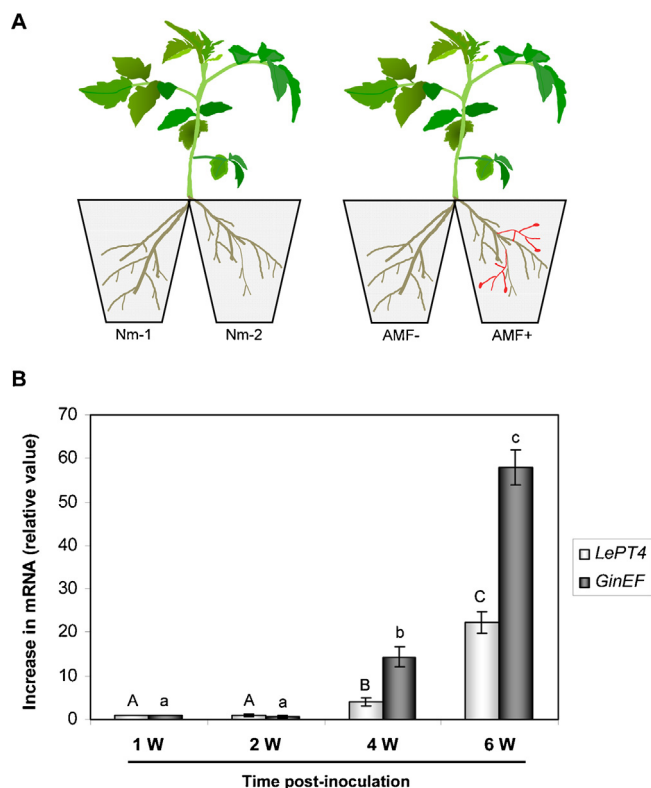
Fig. 2. Effect of AM symbiosis on local and systemic roots from split-root tomato plants over time. (A), Diagram showing the split-root experimental set-up. (B), Gene expression analysis by real time qPCR for the mycorrhizal marker genes LePT4 (white bars) and GinEF (black bars) in local roots (AMF+) of plants colonized by R. irregularis 1, 2, 4 and 6 weeks after inoculation. Expression of each gene after 1 week inoculation was used as reference. Systemic roots (AMF-) exhibited undetectable levels in all cases (data not shown). GinEF , elongation factor from R. irregularis ; LePT4 , tomato phosphate transporter 4. Data points represent the means of three replicates ( \pm SE). Bars with different letters are significantly ( P < 0.05 ) different according to Duncan's multiple range test.
