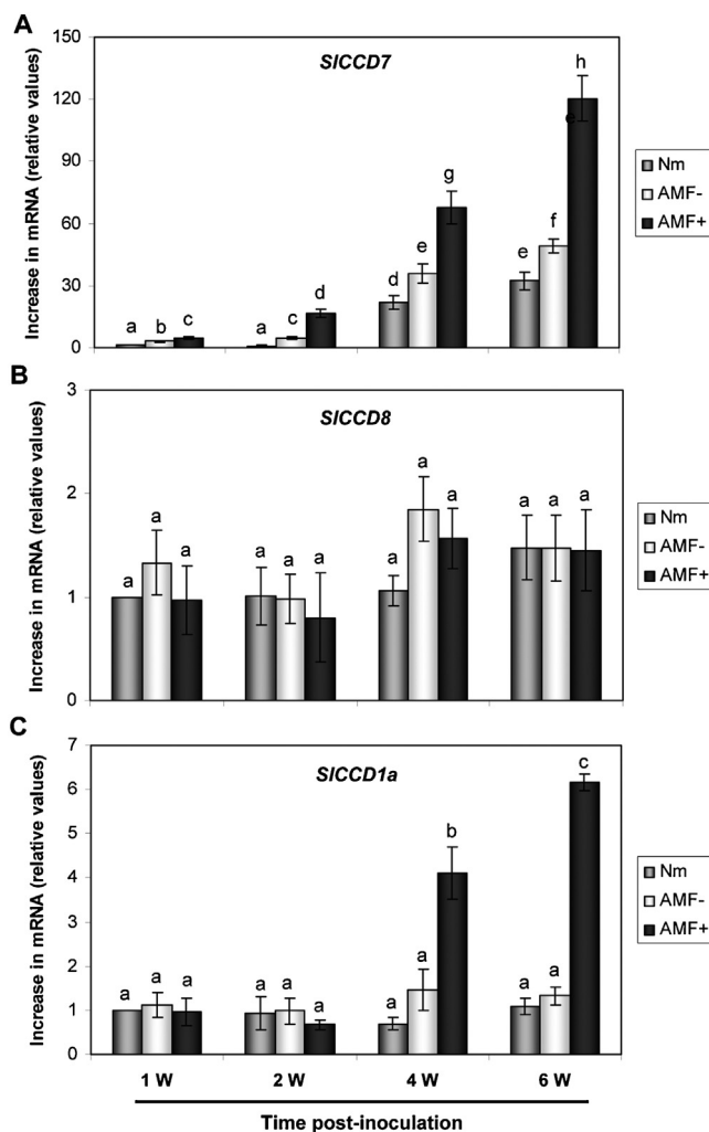
Fig. 4. Transcript level analysis of CCD genes in tomato roots from a split-root system over time. Relative gene expression analysis by real time qPCR for the genes SICCD7 (A), SICCD8 (B) and SICCD1a (C), in roots from non-mycorrhizal plants (Nm, grey bars), and roots with systemic (AMF–, light grey bars) or local effects (AMF+, dark grey bars) from tomato mycorrhizal plants 1, 2, 4 and 6 weeks after inoculation. Expression of each gene in Nm roots after 1 week inoculation was used as reference. Data points represent the means of three replicates ( \pm SE). Bars with different letters are significantly ( P < 0.05 ) different according to Duncan's multiple range test.
