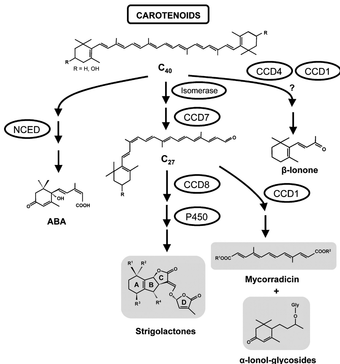
Fig. 1. Apocarotenoid biosynthetic pathways in plants. NCED, 9-cis-epoxycarotenoid dioxygenase; CCD1, CCD4, CCD7 and CCD8 represent carotenoid cleavage dioxygenases 1, 4, 7 and 8, respectively. P450 represents the cytochrome P450 MAX1, involved in SL biosynthesis. Boxes indicate the end-products (SLs, C 13 \alpha -ionol glycoside and C 14 mycorradicin derivatives) analyzed in this study.
