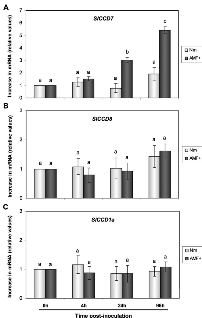
Fig. 5. Analysis of transcript levels of tomato CCD genes during the mycorrhizal pre-symbiotic stage. Relative gene expression analysis by real time qPCR for the genes SICCD7 (A), SICCD8 (B) and SICCD1a (C), in tomato roots after 0, 4, 24 and 96 h after contact with R. irregularis (dark grey bars, AMF+) and corresponding controls without fungus (light grey bars, Nm) in an in vitro system. Expression of each gene after 0 h contact in Nm roots was used as reference. SICCD7 , SICCD8 and SICCD1a , tomato carotenoid cleavage dioxygenases 7, 8 and 1a, respectively. Data points represent the means of three replicates ( \pm SE). Bars with different letters are significantly ( P < 0.05 ) different according to Duncan's multiple range test.
