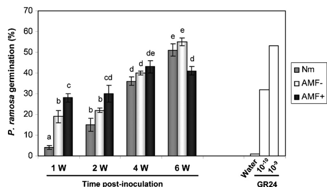
Fig. 3. Influence of mycorrhizal colonization on root-extractable strigolactones quantified by a germination bioassay. Germination of P. ramosa seeds induced by extracts from non-mycorrhizal plants (grey bars, Nm), and systemic (light grey bars, AMF-) and local (dark grey bars, AMF+) roots from tomato mycorrhizal plants 1, 2, 4 and 6 weeks after inoculation. GR24 ( 10^{-9} and 10^{-10} M) and demineralized water were used as positive and negative controls, respectively. Bars represent the means of five independent replicates ( \pm SE). Bars with different letters are significantly ( P < 0.05 ) different according to Duncan's multiple range test.
