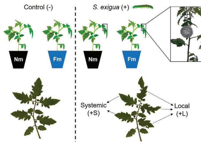
Fig. 1. Experimental set-up and samples used. Harvested shoot material were from Funnelliformis mosseae -colonized (Fm) or non-mycorrhizal (Nm) tomato plants, infested (+) or not (-) with Spodoptera exigua . Two second instar larvae were placed into a clip-cage per plant. Clip-cages were moved every day into new leaflets and larval mortality was recorded daily, for two weeks. At the end of the assay, shoot material was collected from each treatment, differentiated into leaflets from non-stressed plants (control; -), leaflets with damage from S. exigua feeding (local, +L) and those leaflets without damage but contiguous to where S. exigua fed (systemic, +S).
